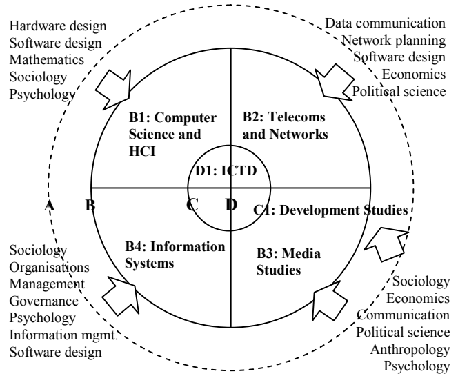
Fig. 1. ICTD subdisciplines
